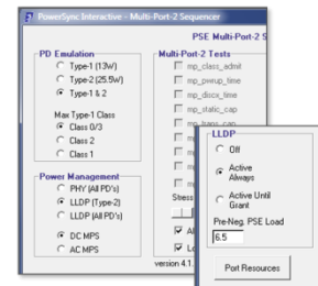
LLDP Enabling in PSE Multi-Port Suite
