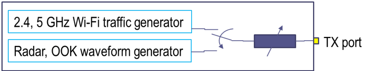
iGen block diagram
