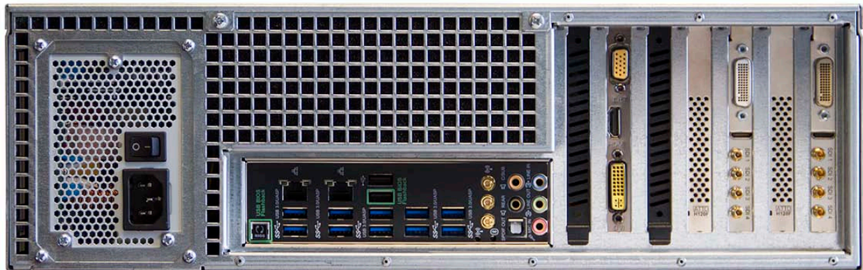
Figure 6: RTM 4K Back Panel (Supplied with two sets of Quad SMB to BNC conversion cables for inputs 1 and 2 and mini HDMI cables for error recording playback from either or both outputs) Models: RTM-S8084 (10 TB storage model) or RTM-8084-5 (5 TB storage model)
