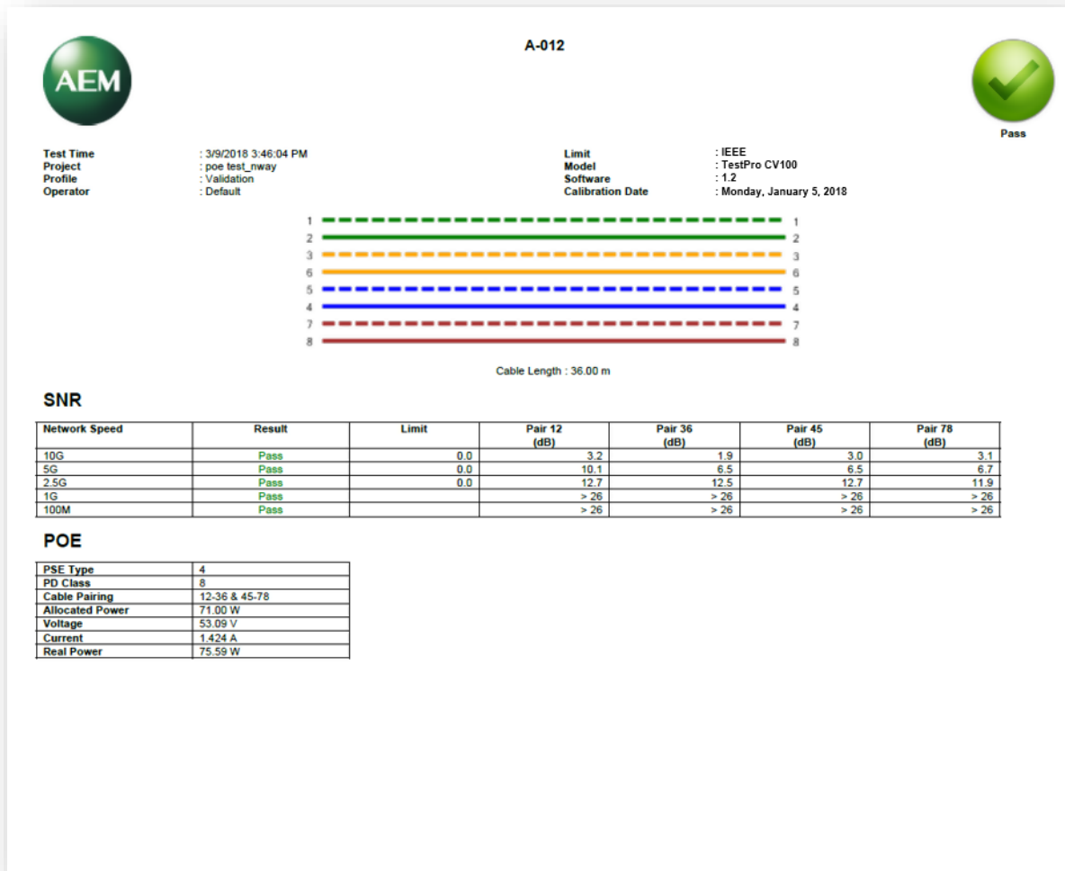
Figure 7: PoE and Multi-gig Verification Test Report
