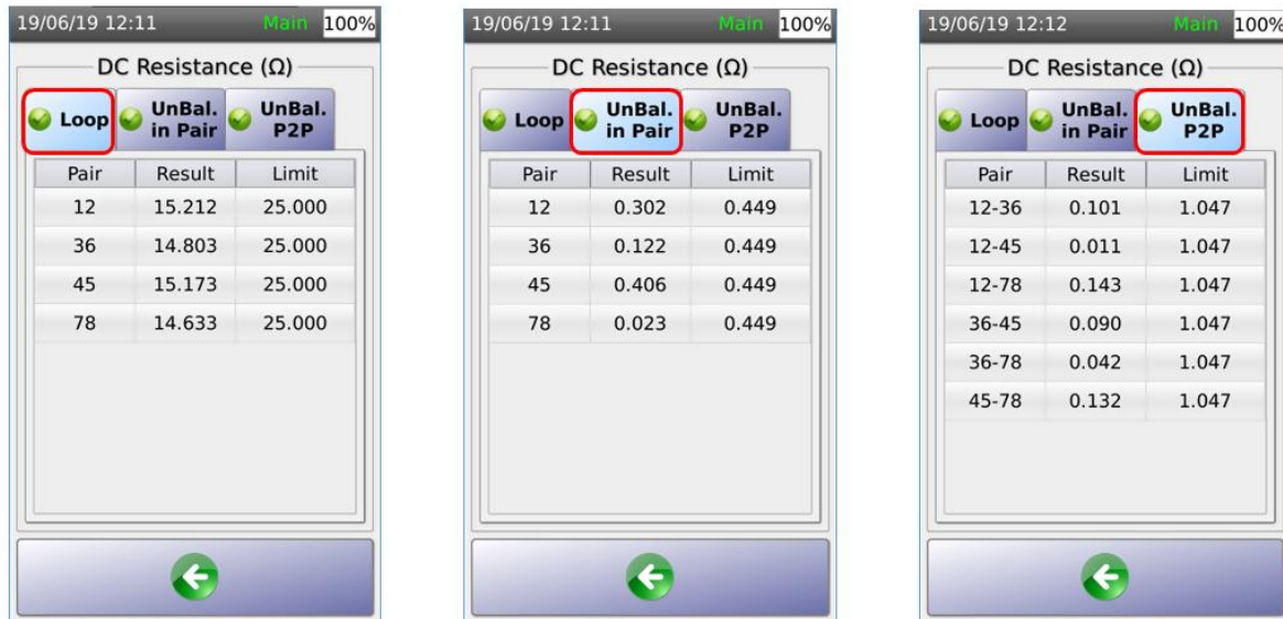
Figure 6: Resistance and Resistance Unbalance Measurement
