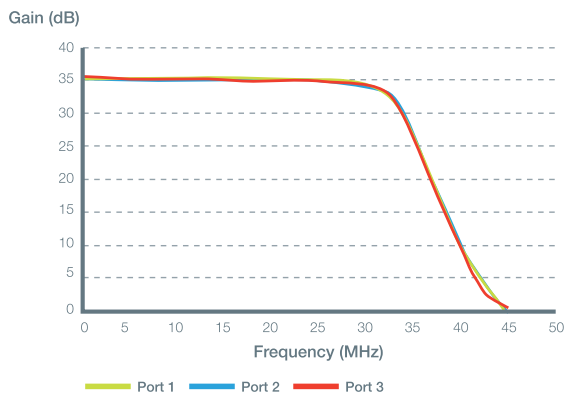
Amplifier gain
