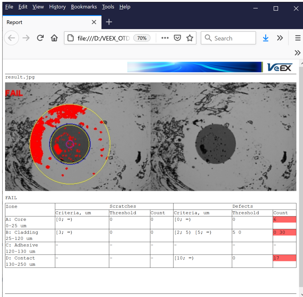
Fiberscope test viewed in an HTML browser
