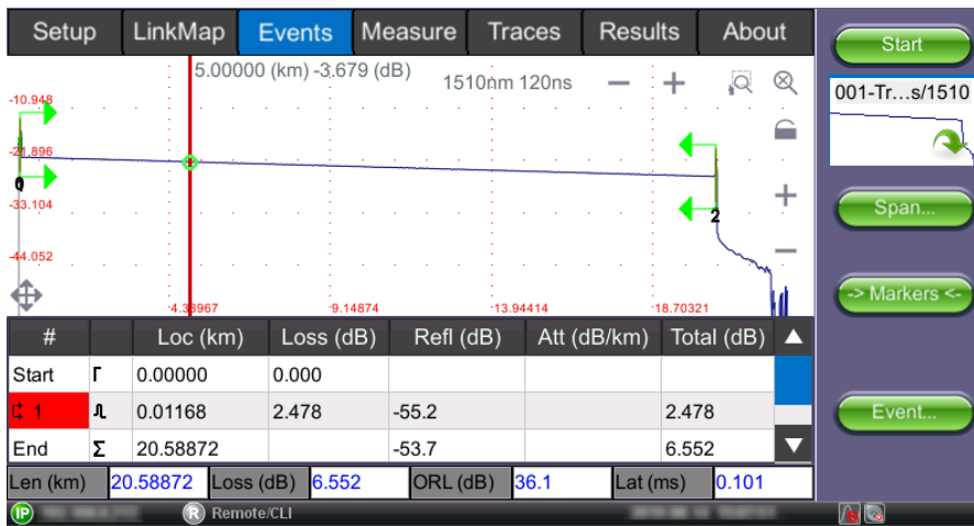
Event Table (RXT-4113)
