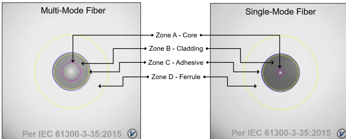
Cross-section-mode and multi-mode fiber zones
