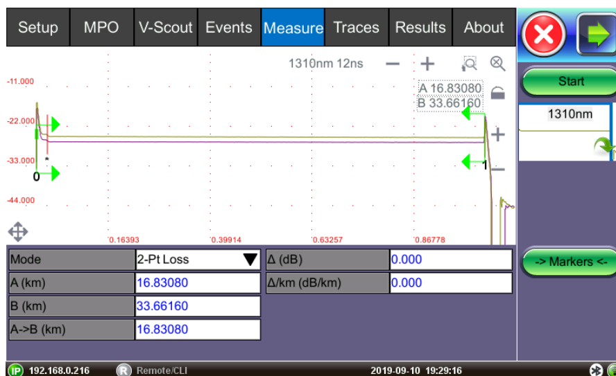
Splice Loss using 2-Point LSA method (MPO)
