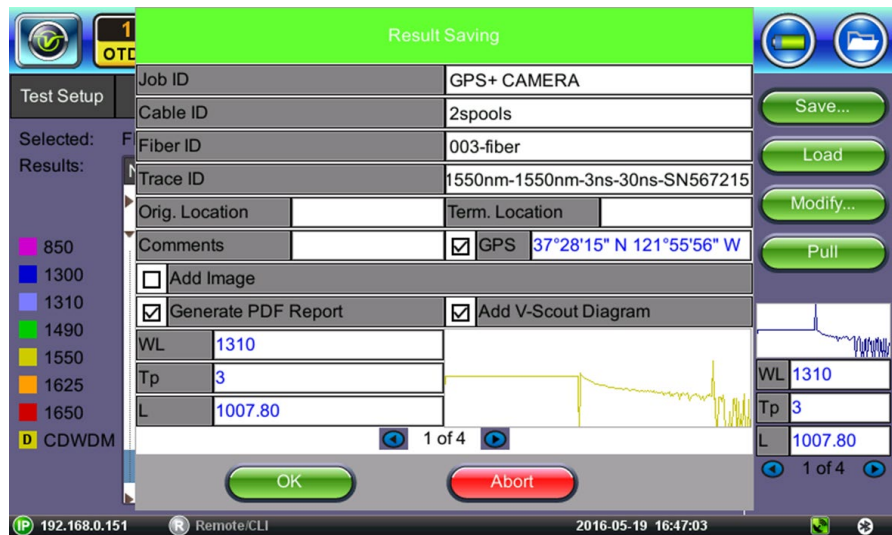
MTTplus Manual Save: Image added to results
