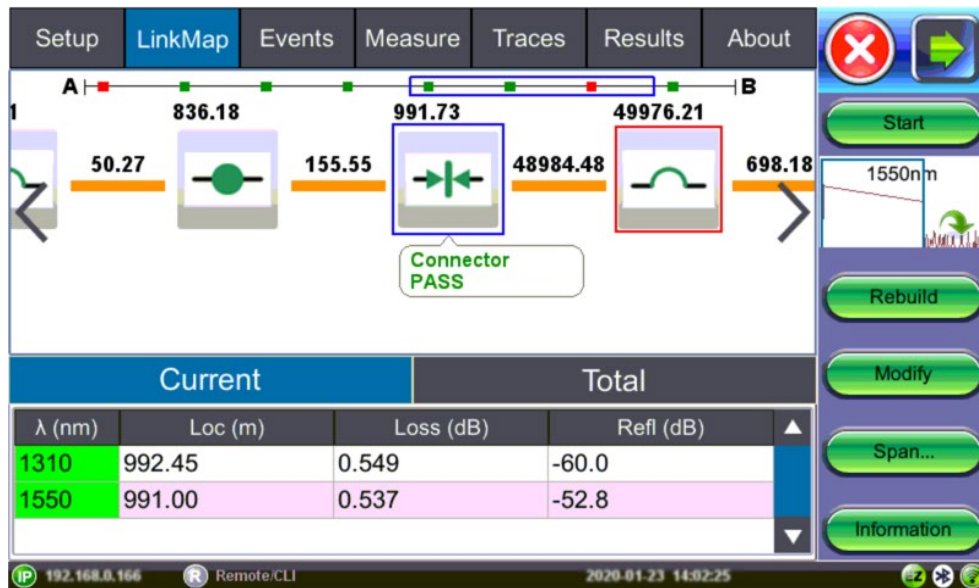
V-Scout Link Map
