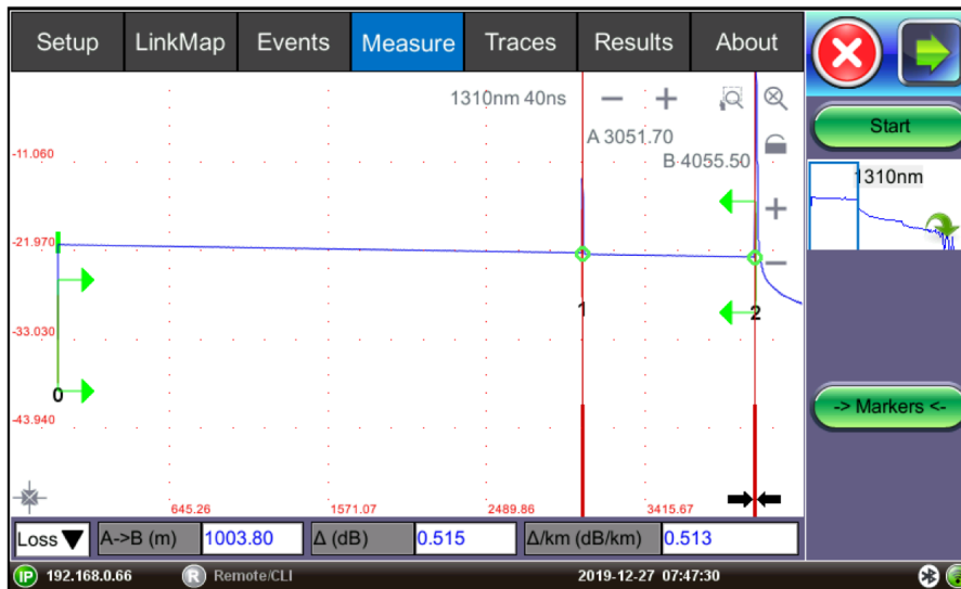
Distance measurement -measure expanded trace view
