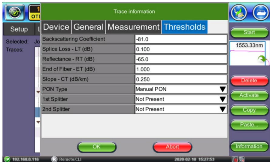
Trace Information - Thresholds
