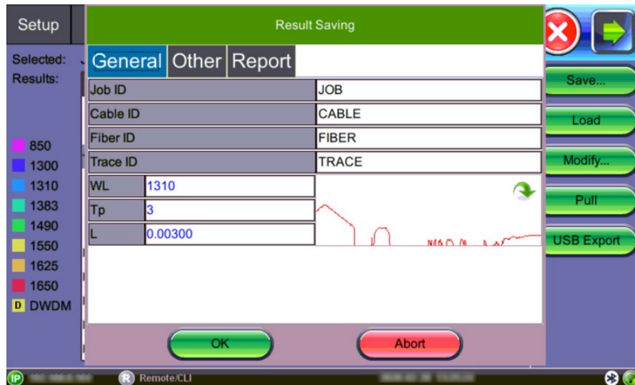
OTDR Traces: Result Saving Window
