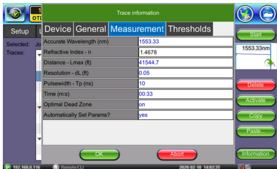
Trace Information - Measurement
