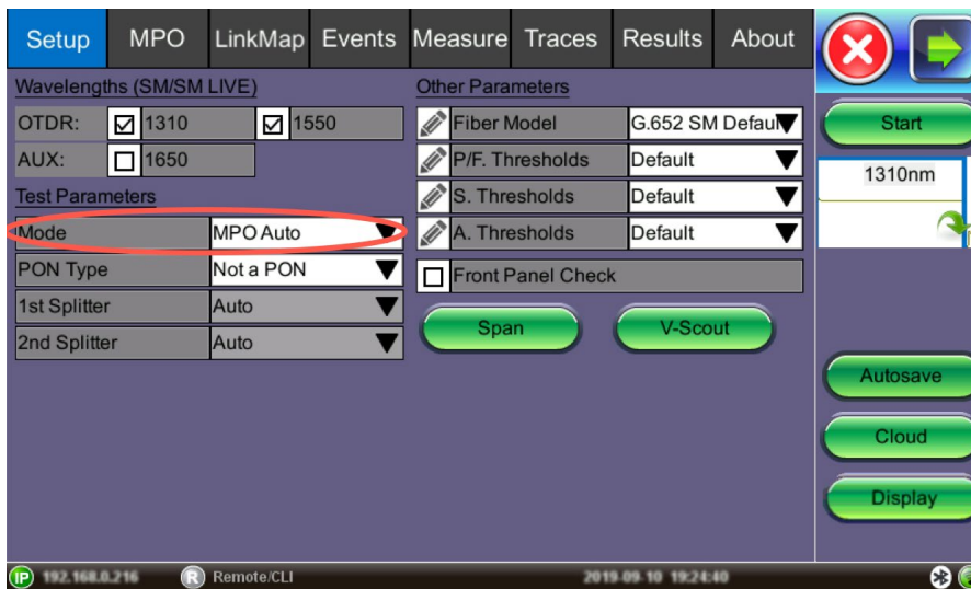
MPO Auto Setup
