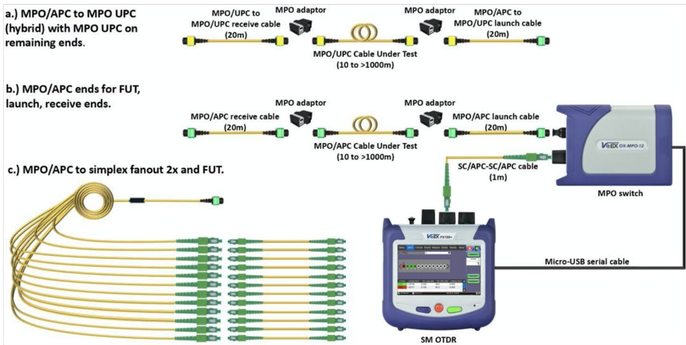
OX-MPO-12: Example of Connections
