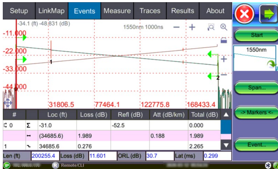
Bidirectional test: Events view
