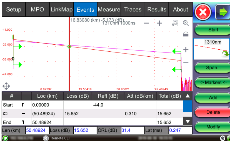
Event Table - MPO test
