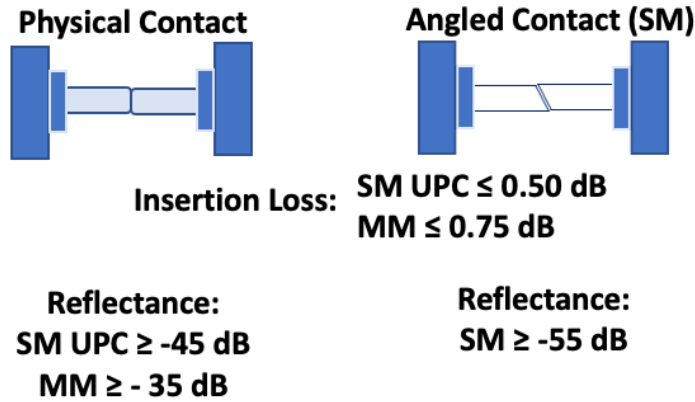
UPC and APC return loss
