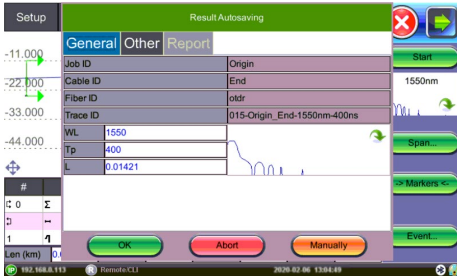
Autosave Results screen
