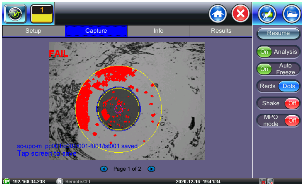
Real time video of the connector face. Red contours indicate scratches and defects.
