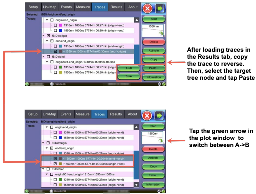
Bidirectional testing: Traces tab
