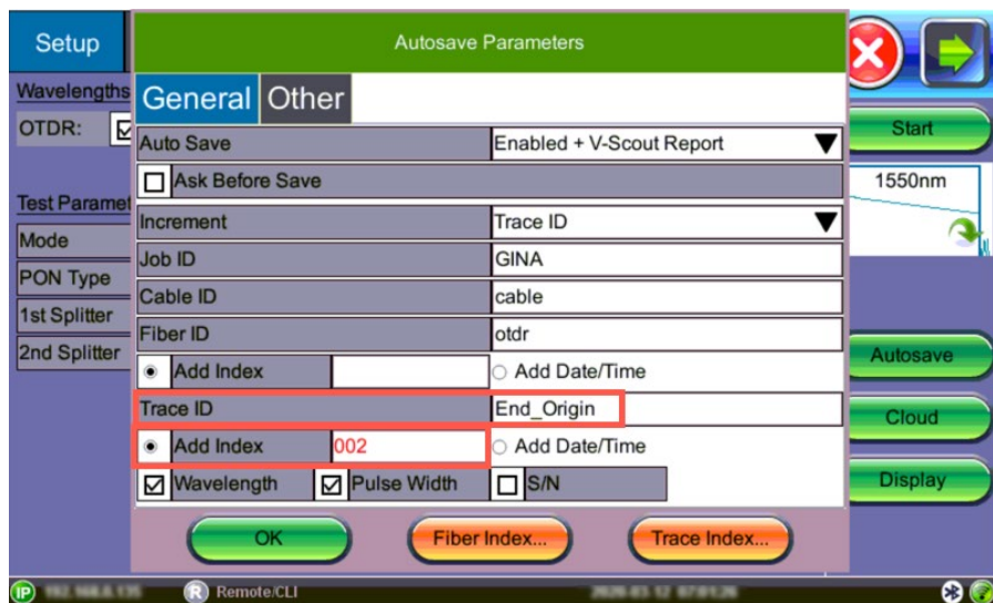
Bidirectional Trace - Reverse Direction testing
