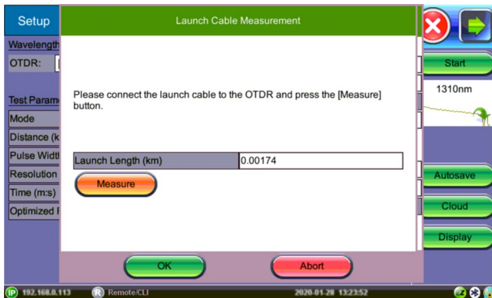
OTDR Setup: Auto Measure Cables
