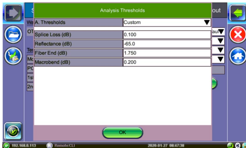
OTDR Setup: Analysis Thresholds
