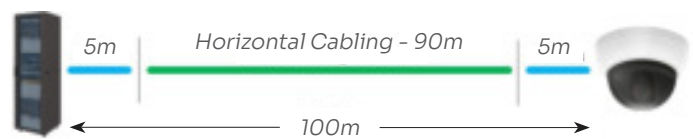
Figure 3 : Twisted Pair Ethernet Maximum Length
