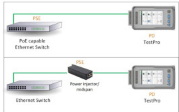
Figure 1: PoE PSE switch/midspan with TestPro acting as a PD
